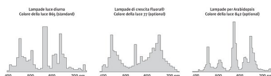
Light Spectra
